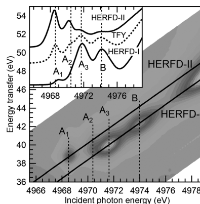
Figure 3. 1s3p RIXS plane of Ti K-edge pre-edge of N- \text{TiO}_2 . 1s3p RIXS plane is obtained by collecting Ti K_\beta fluorescence while scanning the Ti K-edge with the incident X-ray beam. HERFD-I and HERFD-II cuts are shown with solid black lines. Inset: the pre-edge region of the Ti K-edge spectrum for N- \text{TiO}_2 measured in TFY, HERFD-I, and HERFD-II.
